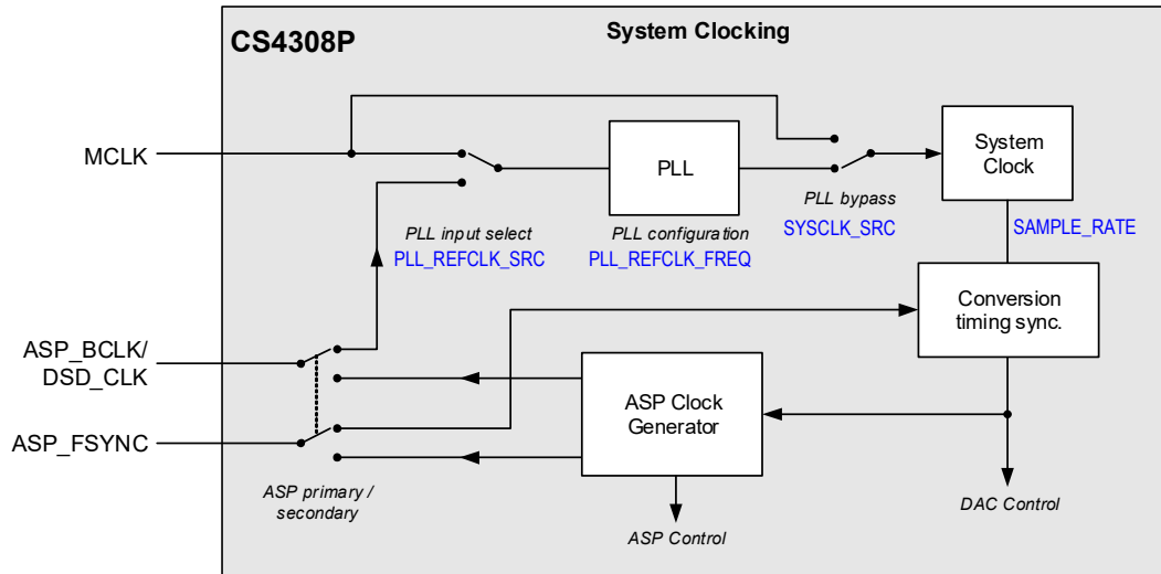
Figure 4-1. System Clocking
