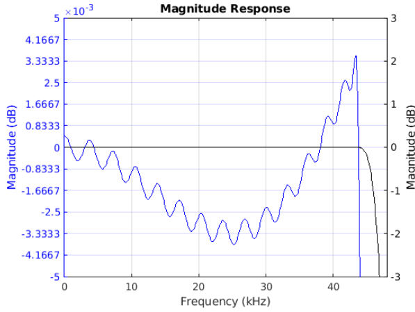
Figure 7-19. Passband Magnitude
